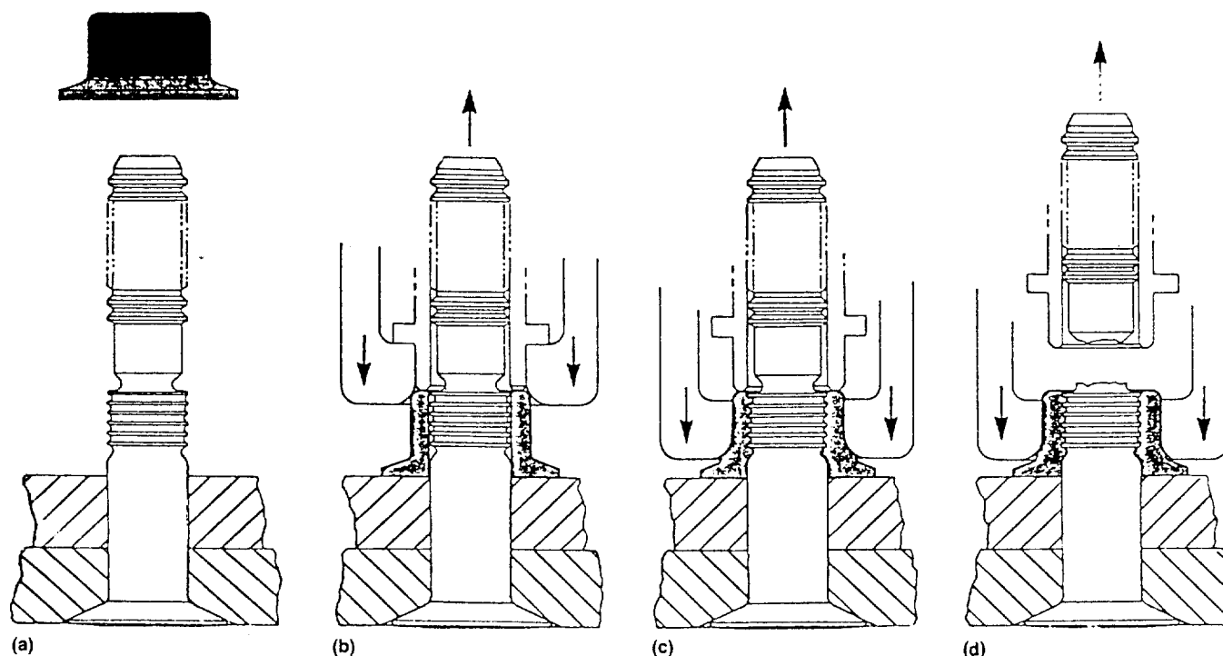
(a) Flanged collar is placed over lightweight pin. (b) Installation tool grips and pulls pin, drawing sheets tightly together and removing sheet gap. (c) As pull on pin increases, tool anvil swages flanged collar into locking grooves and forms permanent vibration-resistant lock. (d) Pull on pin continues until pin fractures at breakneck groove and is then ejected. Tool anvil disengages swaged collar.
