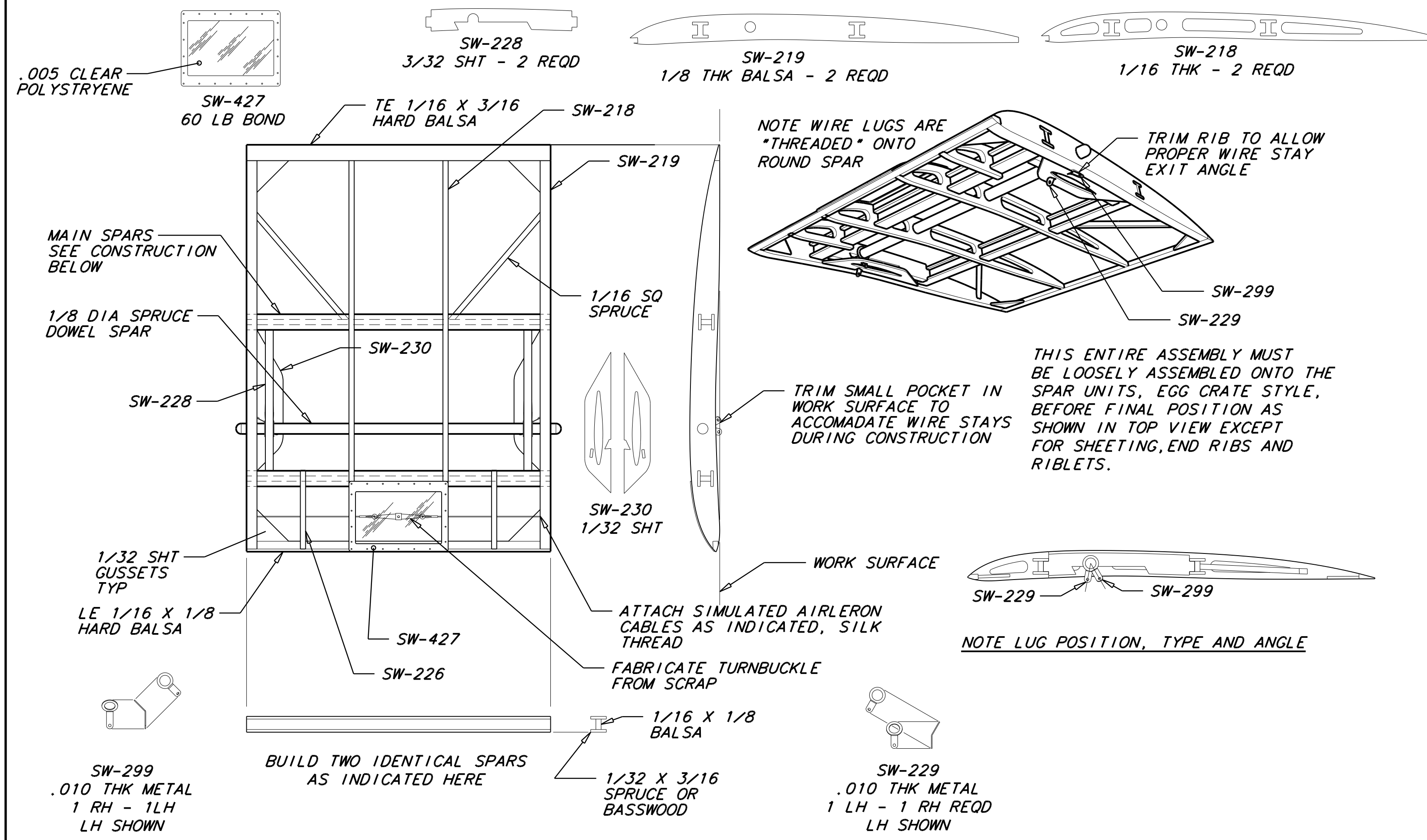
TOP SUB-WING ASSEMBLY
