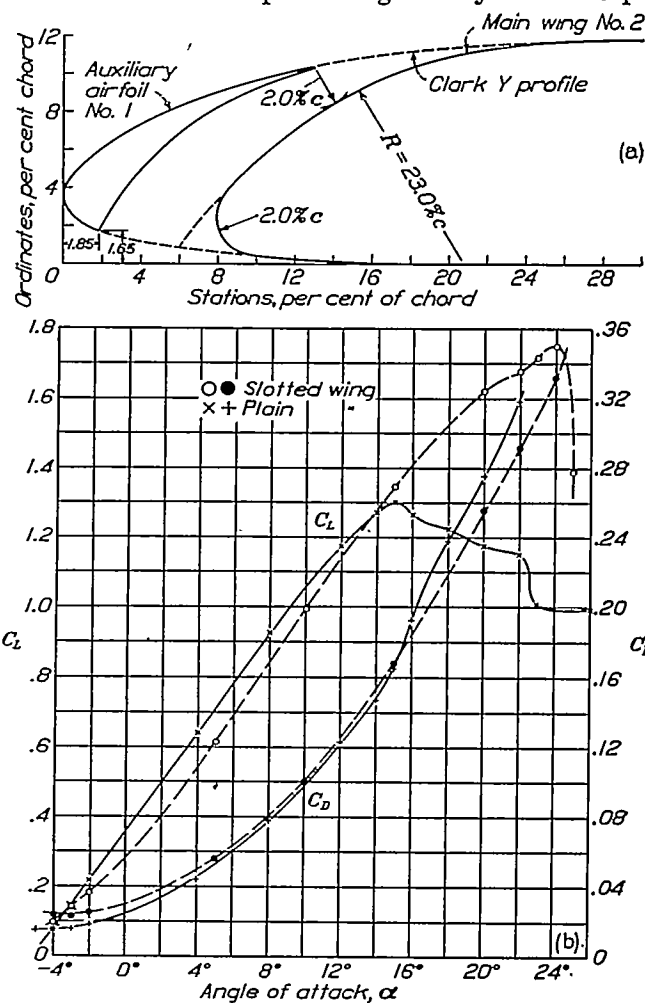
FIGURE 4.—Characteristics of Clark Y wing with best fixed slot
