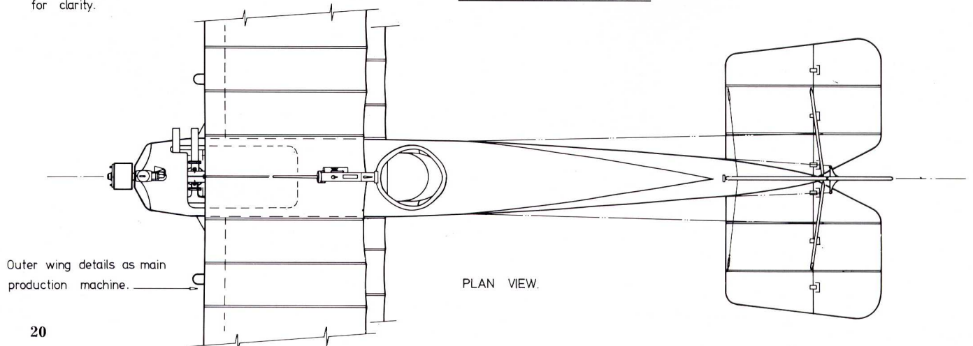
EARLY PRODUCTION MACHINE.
